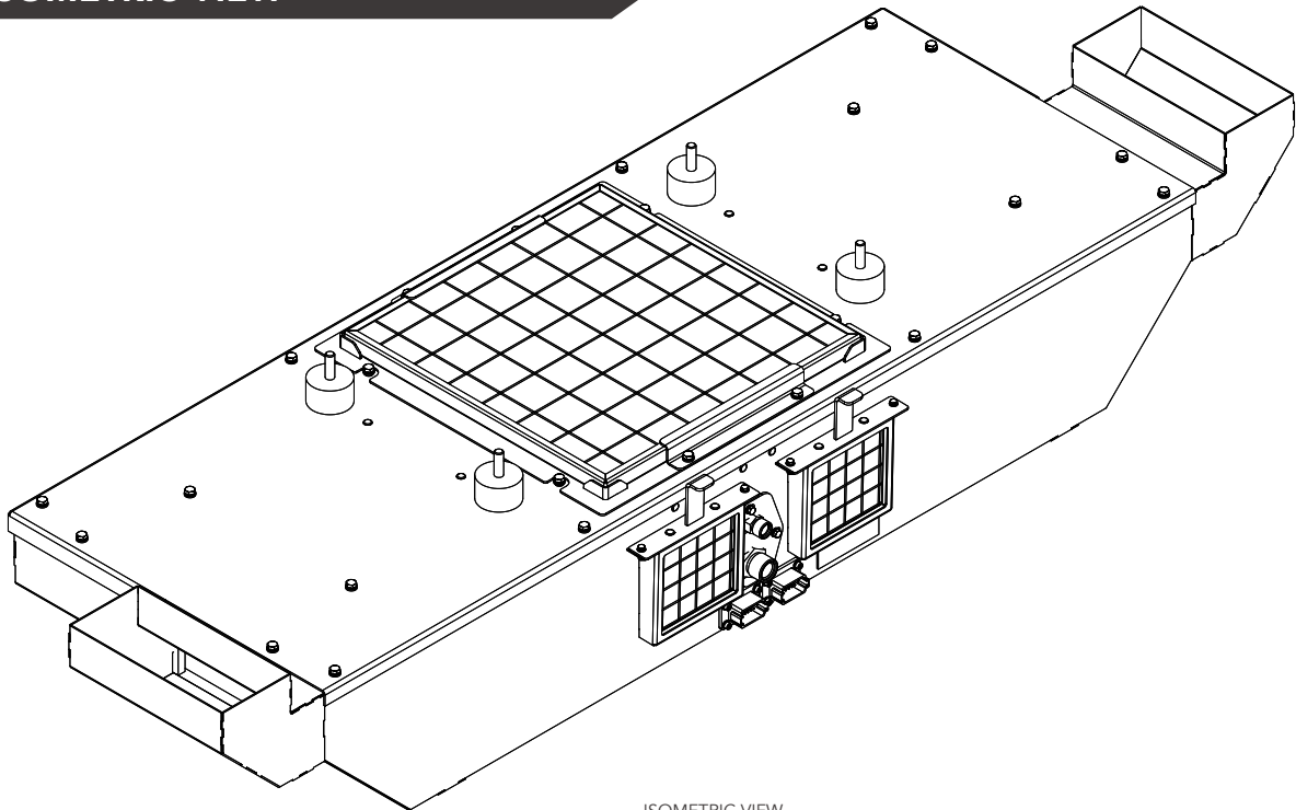
ISOMETRIC VIEW
